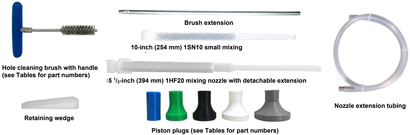
FIGURE 5— EF600 ADHESIVE INSTALLATION ACCESSORIES
