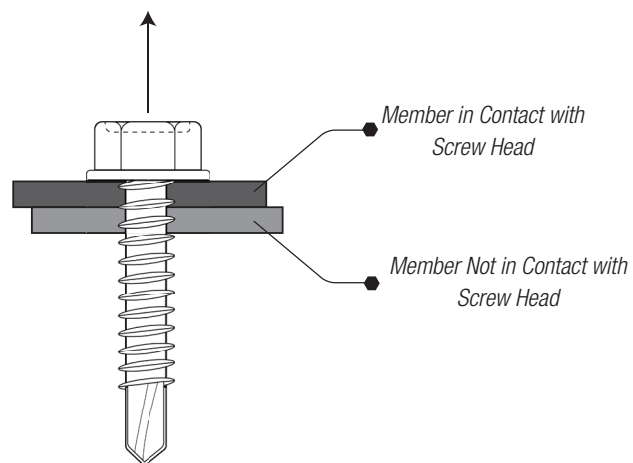
TENSION PULL-OUT
