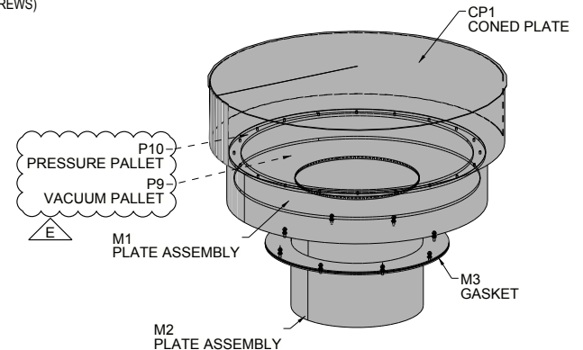
ISOMETRIC VIEW 14AFFFTV24
