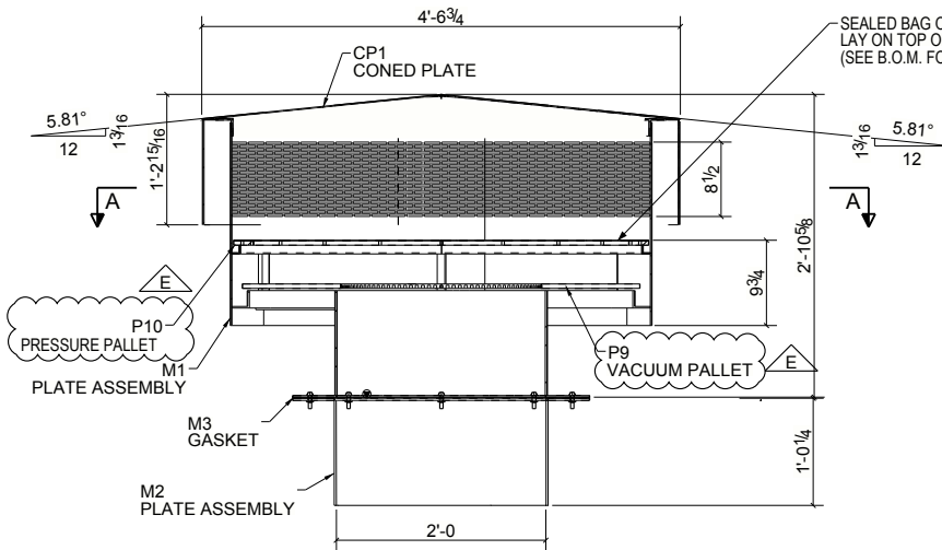
ELEVATION VIEW
