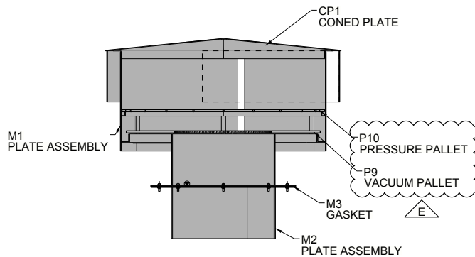
ELEVATION VIEW
