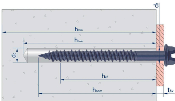
FIGURE 2: LENGTH IDENTIFICATION SYSTEM
